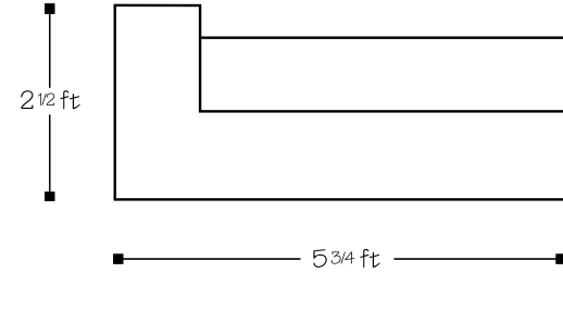
Measurements for Foot Rail for the Bar
